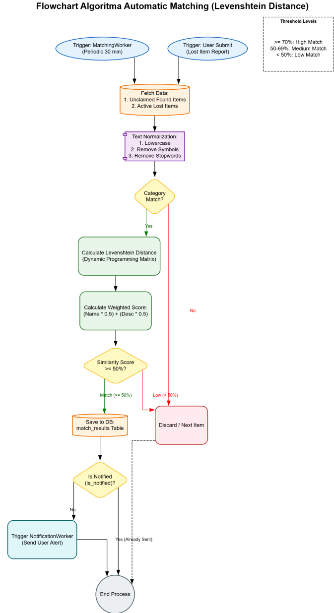
Fig. 5. Automatic Matching Algorithm Workflow
